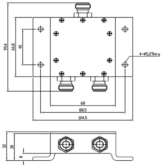
Mounting Details
