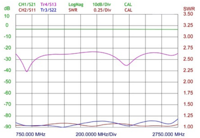
Typical response curve
