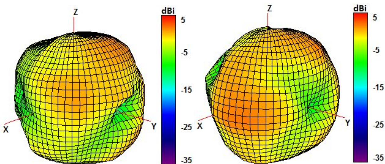
Cable 1: CELLULAR/LTE
